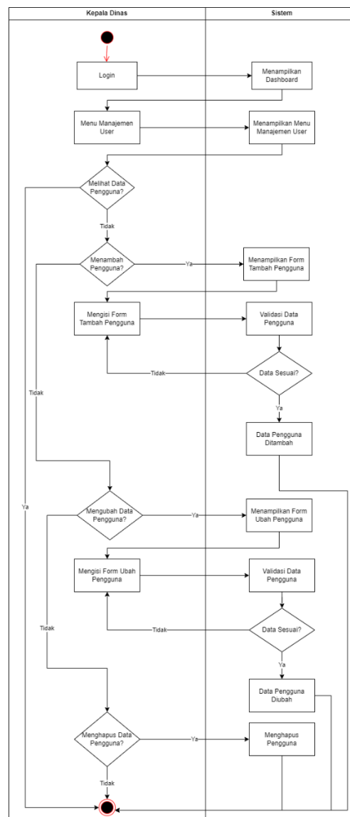
Gambar 3.7 Activity diagram manajemen user
